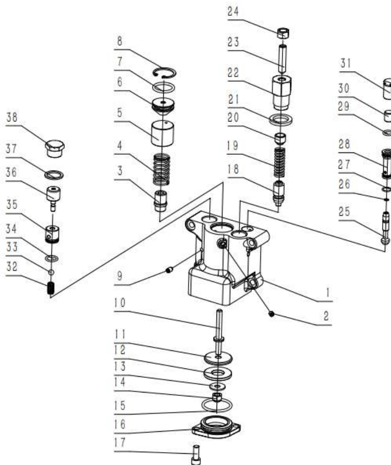
Pic5 Intake Valve assy
