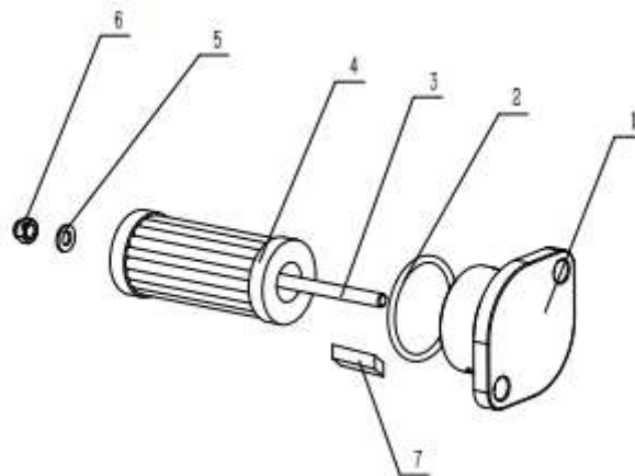
Pic3 Oil filter Assy
