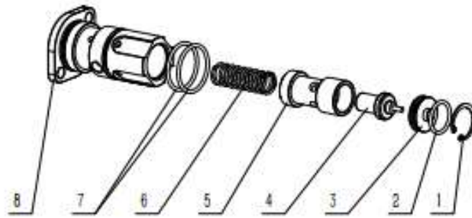
Pic6 Thermal valve assy
