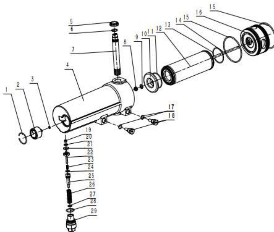
Pic7 Oil Separator Assy
