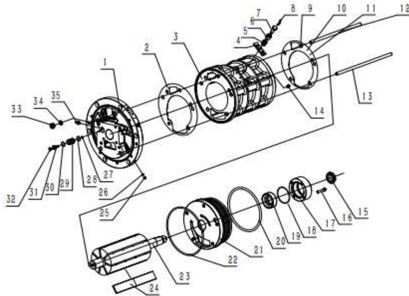
Pic4 Rotor&amp;stator assy
