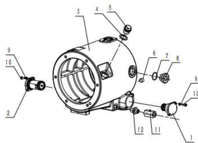
Pic2 Oil Cover Assy
